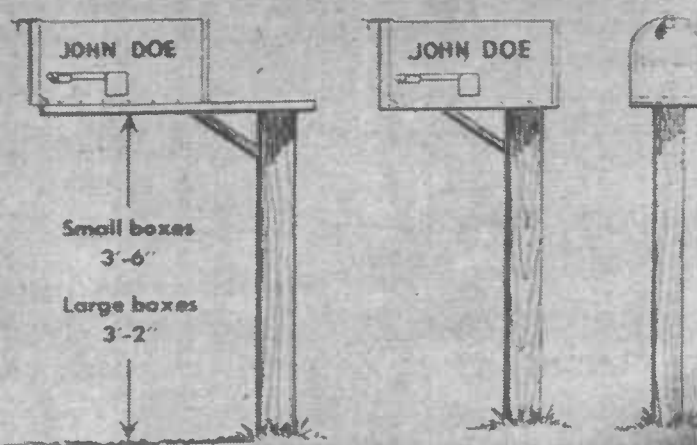
SUGGESTED INSTALLATIONS OF SINGLE BOX
